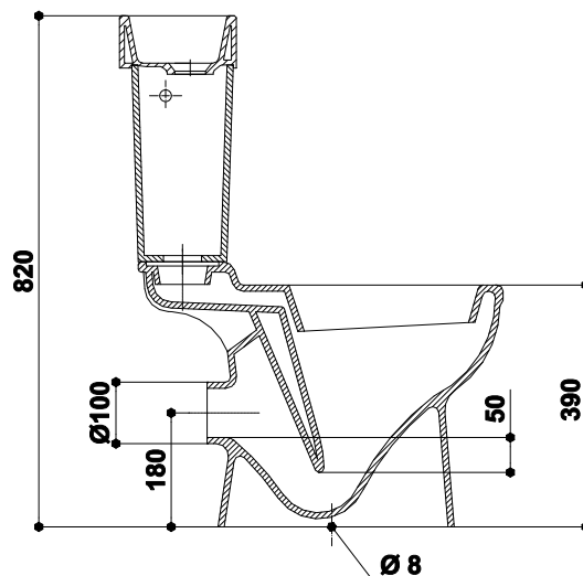
VAS WC DUO PACK WC BOWL DWO PACK ТУАЛЕТ ПАК
